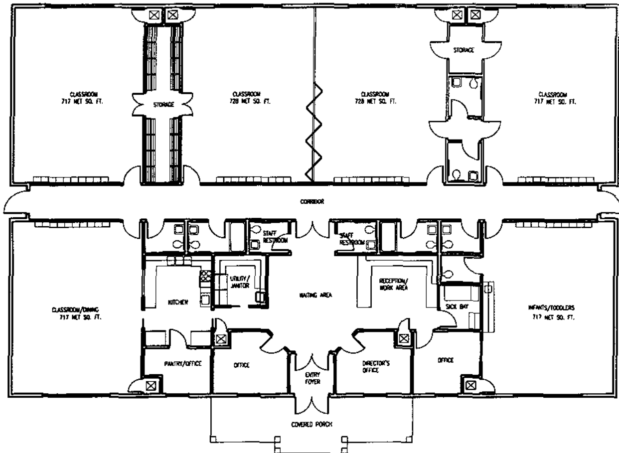
PRELIMINARY FLOOR PLAN – 7,525 GROSS HEATED SQ. FT.
